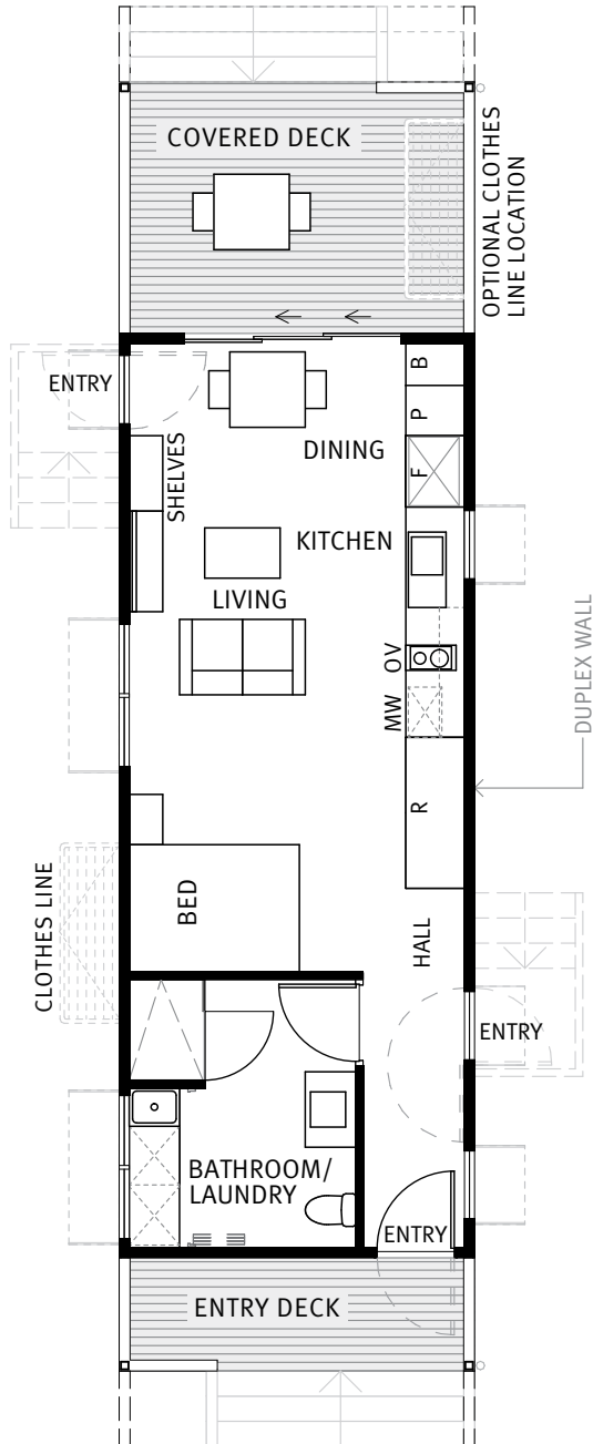
FLOOR PLAN SCALE 1:100 at A4
